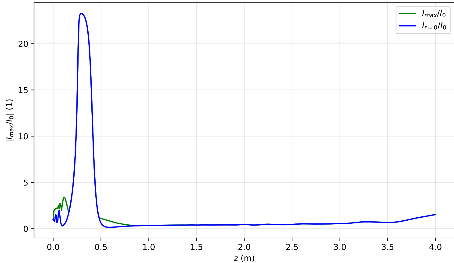
I_{max}(x = 0, y = 0, z)/I_0 , Pin=3.0P_{cr} , artificial time
